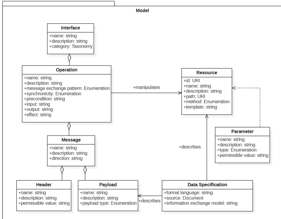
Figure 4 Package Model
